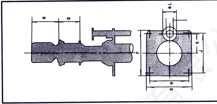
安装平面图 Plane graph of installation
